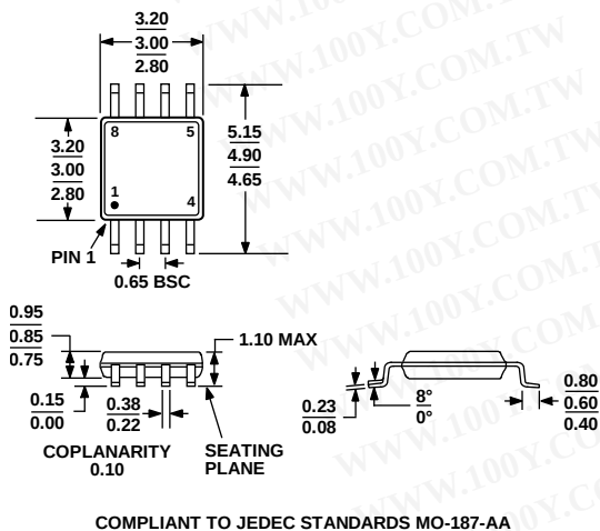
Figure 52. 8-Lead Mini Small Outline Package [MSOP] (RM-8)
