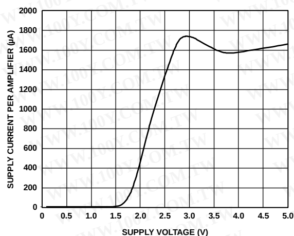
Figure 19. Supply Current per Amplifier vs. Supply Voltage
