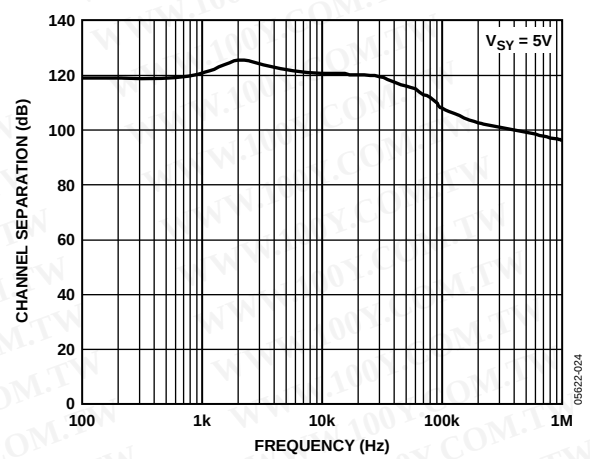
Figure 27. Channel Separation
