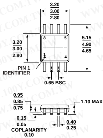
Figure 38. 8-Lead Mini Small Outline Package [MSOP] (RM-8)
