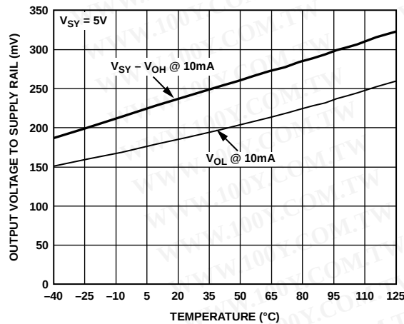
Figure 14. Output Voltage to Supply Rail vs. Temperature ( I_L = 10mA )
