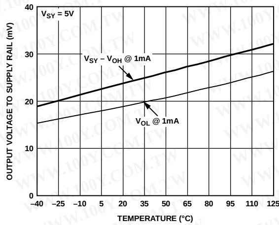
Figure 13. Output Voltage to Supply Rail vs. Temperature ( I_L = 1mA )
