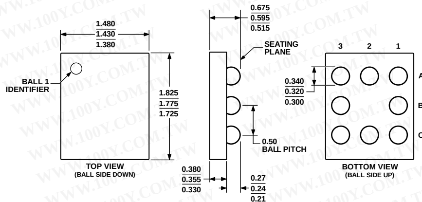
Figure 61. 8-Ball Wafer Level Chip Scale Package [WLCSF] (CB-8-1) Dimensions shown in millimeters
