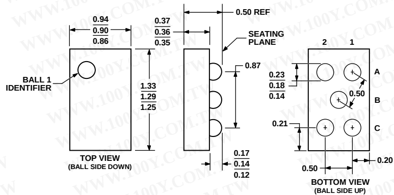
Figure 57. 5-Ball Wafer Level Chip Scale Package [WLCSP] (CB-5-1)
