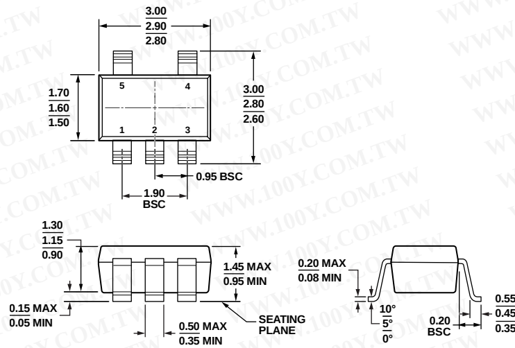
COMPLIANT TO JEDEC STANDARDS MO-178-AA Figure 58. 5-Lead Small Outline Transistor Package [SOT-23] (RJ-5)
