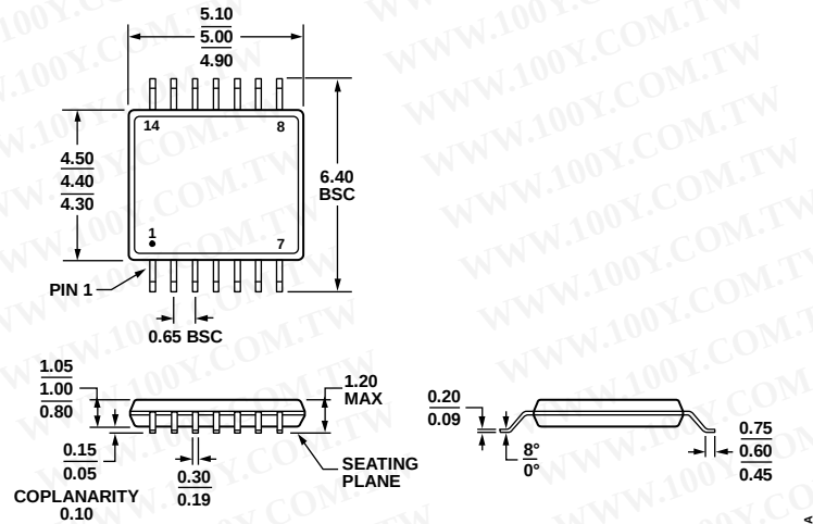
Figure 66. 14-Lead Thin Shrink Small Outline Package [TSSOP] (RU-14)
