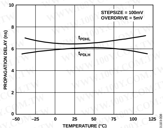
Figure 8. Propagation Delay, t_{PDHL}/t_{PDL} vs. Temperature
