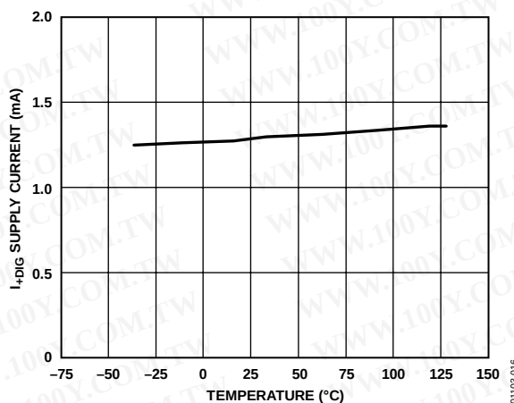
Figure 16. I+DIG Supply Current/Comparator vs. Temperature
