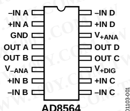
Figure 2. 16-Lead Narrow Body SOIC (R-16)
