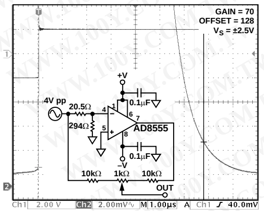
Figure 46. Settling Time 0.1%
