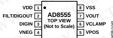
Figure 2. 8-Lead SOIC (Not Drawn to Scale)
