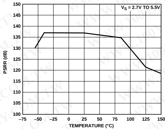
Figure 35. PSRR vs. Temperature
