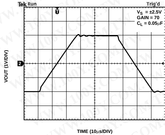
Figure 40. Large Signal Response
