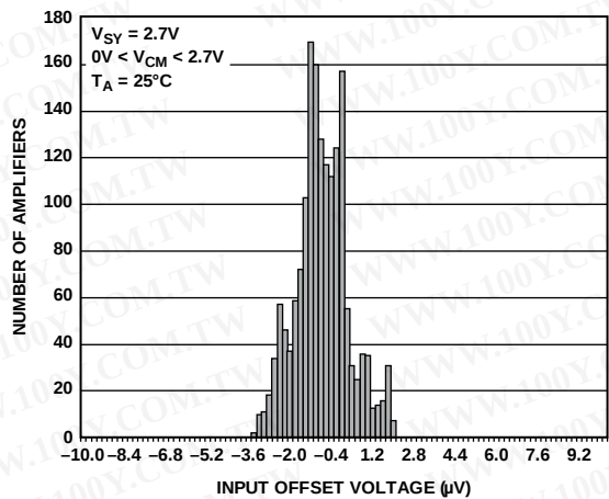
Figure 26. AD8538 Input Offset Voltage Distribution
