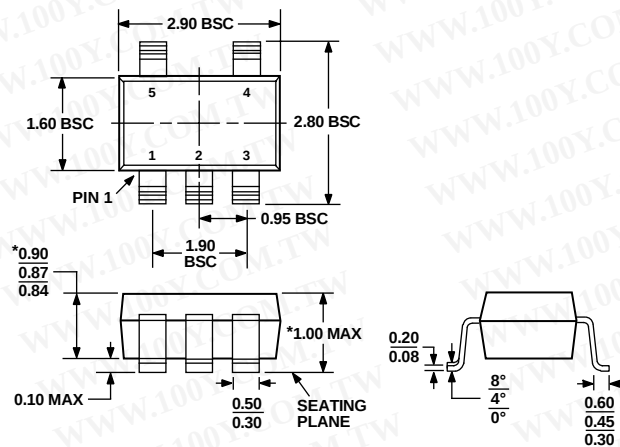
Figure 64. 5-Lead Thin Small Outline Transistor Package [TSOT-23] (UJ-5)
