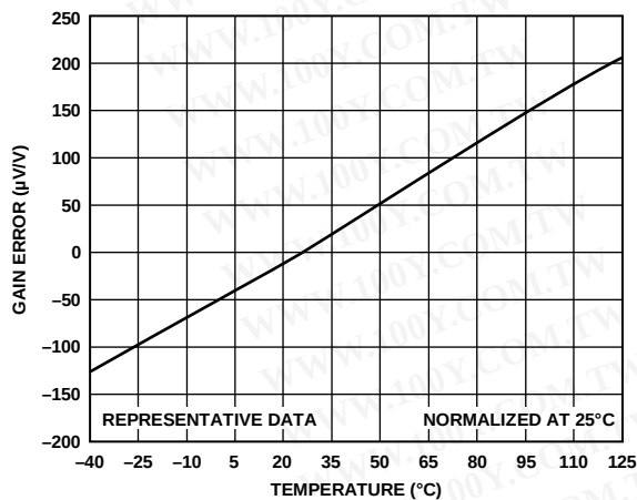
Figure 17. Gain Error vs. Temperature, Normalized at 25 ^{\circ}C
