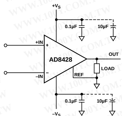
Figure 40. Supply Decoupling, REF, and Output Referred to Local Ground
