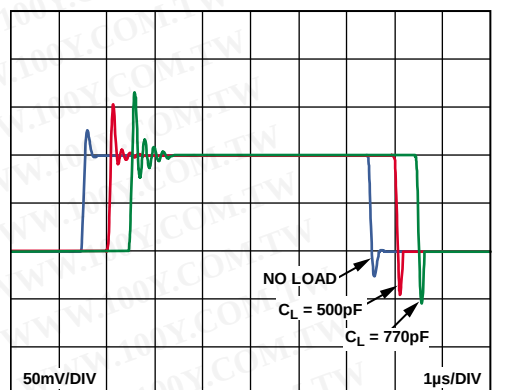
Figure 35. Small Signal Pulse Response with Various Capacitive Loads, No Resistive Load
