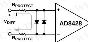
Figure 43. Protection for Large Differential Voltages
