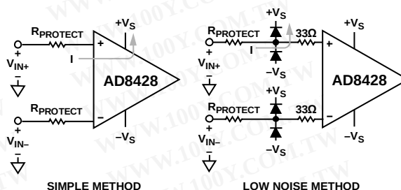
Figure 42. Protection for Voltages Beyond the Rails
