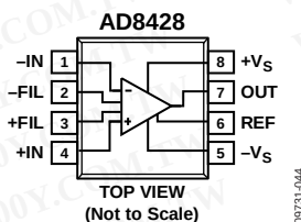
Figure 39. Pinout Diagram
