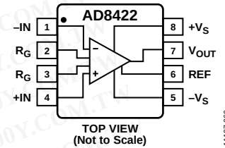
Figure 59. Pinout Diagram
