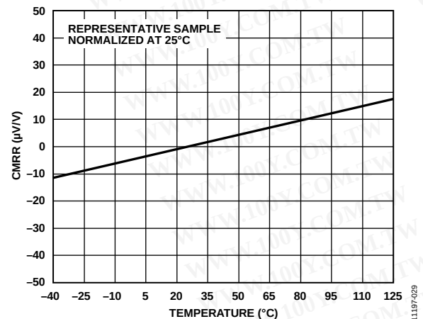
Figure 30. CMRR vs. Temperature (G = 1), Normalized at 25°C
