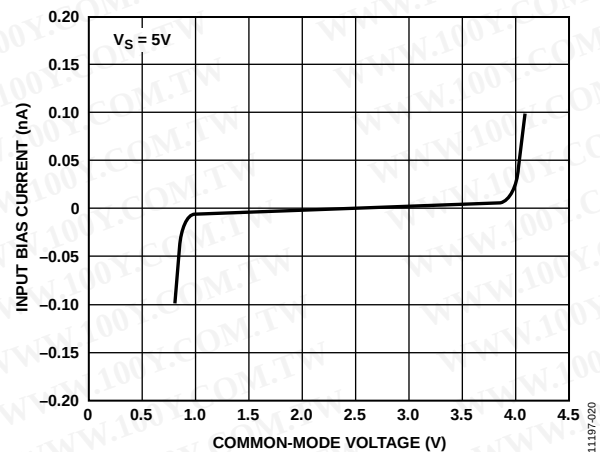
Figure 21. Input Bias Current vs. Common-Mode Voltage, V_S = 5\text{ V}
