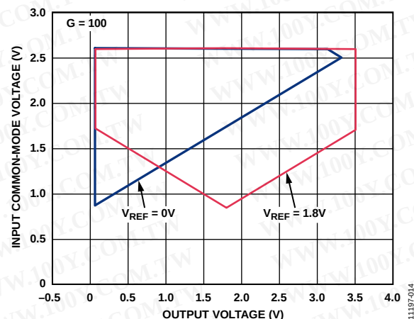
Figure 15. Input Common-Mode Voltage vs. Output Voltage ( G = 100 ), Single-Supply, V_S = 3.6\text{ V}
