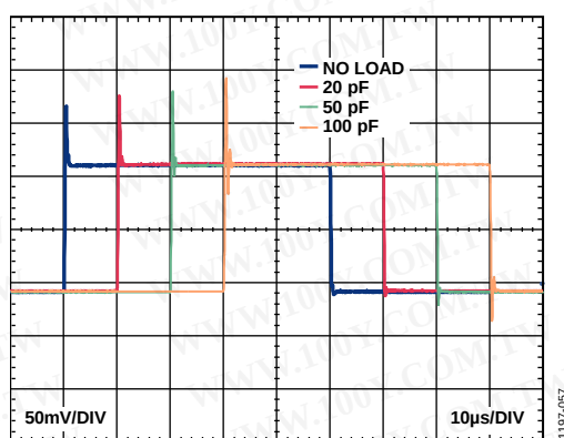
Figure 56. Small Signal Pulse Response with Various Capacitive Loads ( G = 1 ), R_L = \text{No Load}
