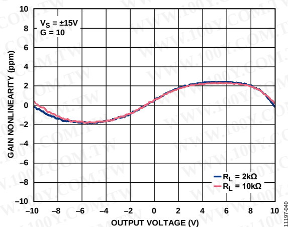
Figure 39. Gain Nonlinearity ( G = 10 )
