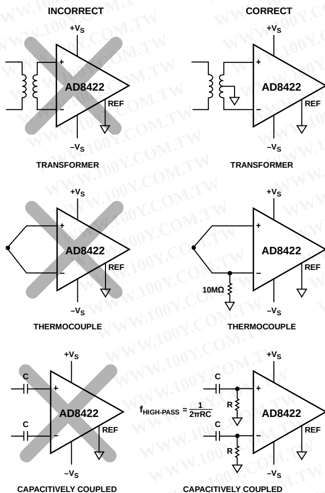
Figure 61. Creating an Input Bias Current Return Path
