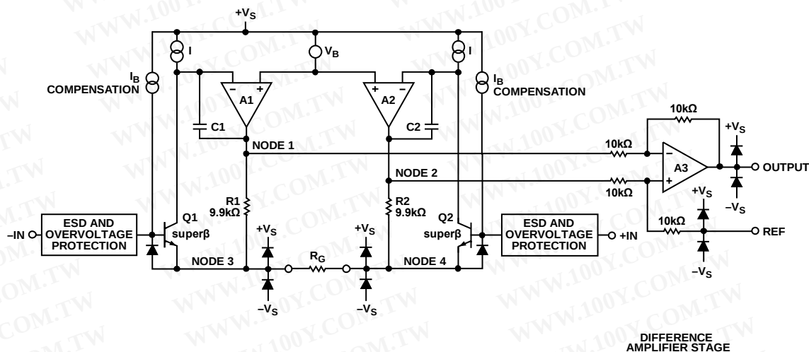
Figure 57. Simplified Schematic
