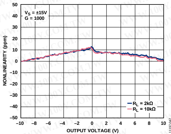
Figure 41. Gain Nonlinearity (G = 1000)
