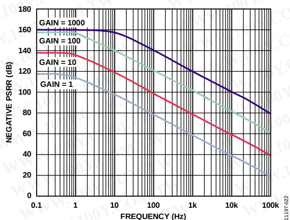
Figure 23. Negative PSRR vs. Frequency
