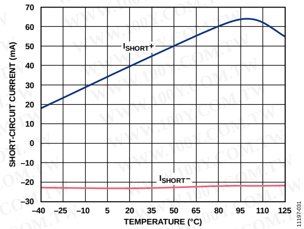
Figure 32. Short-Circuit Current vs. Temperature (G = 1)
