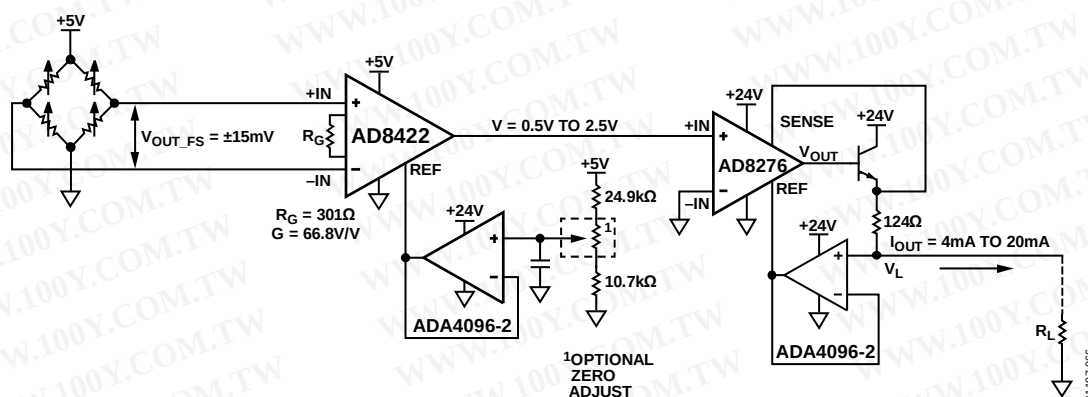
Figure 65. Bridge Circuit with 4 mA to 20 mA Output
