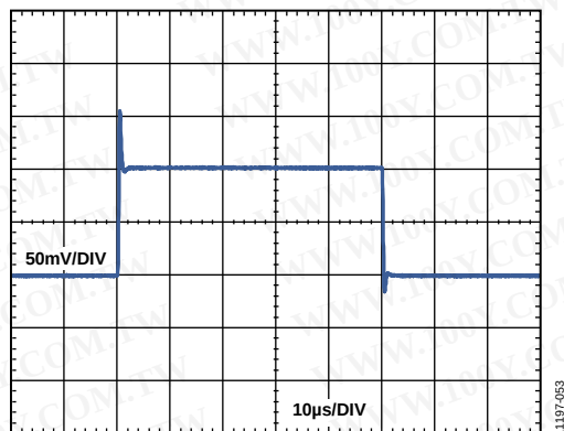
Figure 52. Small Signal Pulse Response ( G = 1 ), R_L = 2\text{ k}\Omega , C_L = 100\text{ pF}
