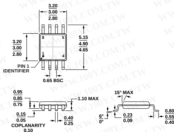
Figure 68. 8-Lead Mini Small Outline Package [MSOP]
