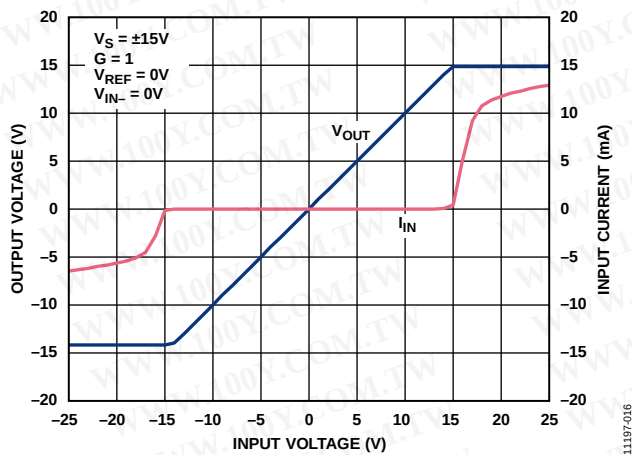
Figure 17. Input Overvoltage Performance; G = 1 , V_S = \pm 15\text{ V}
