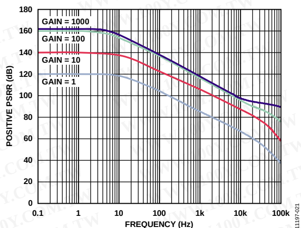
Figure 22. Positive PSRR vs. Frequency
