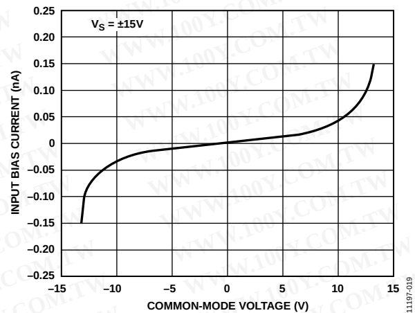
Figure 20. Input Bias Current vs. Common-Mode Voltage, V_S = \pm 15\text{ V}
