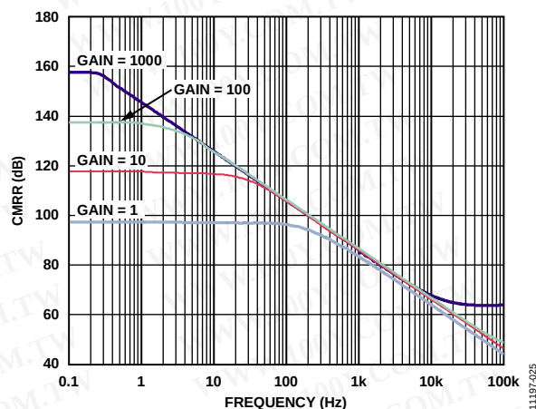
Figure 26. CMRR vs. Frequency, 1 kΩ Source Imbalance
