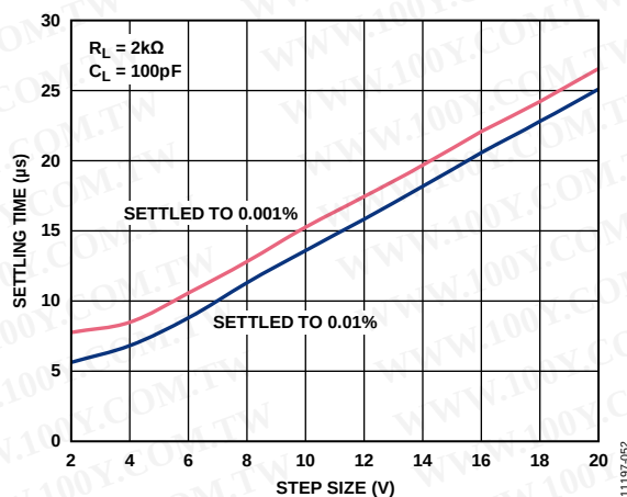
Figure 51. Settling Time vs. Step Size ( G = 1 )
