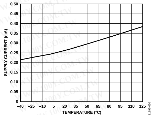
Figure 31. Supply Current vs. Temperature (G = 1)
