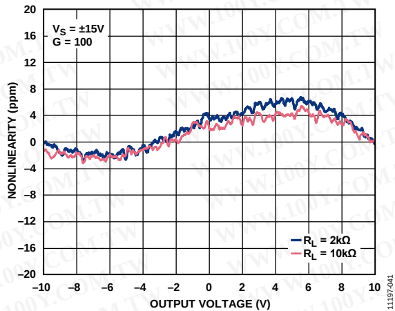
Figure 40. Gain Nonlinearity (G = 100)
