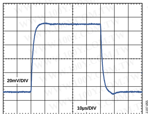
Figure 54. Small Signal Pulse Response ( G = 100 ), R_L = 2\text{ k}\Omega , C_L = 100\text{ pF}
