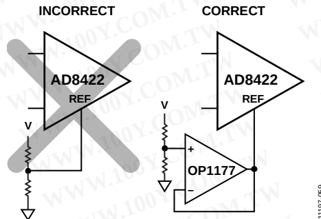
Figure 58. Driving the Reference Pin (REF)
