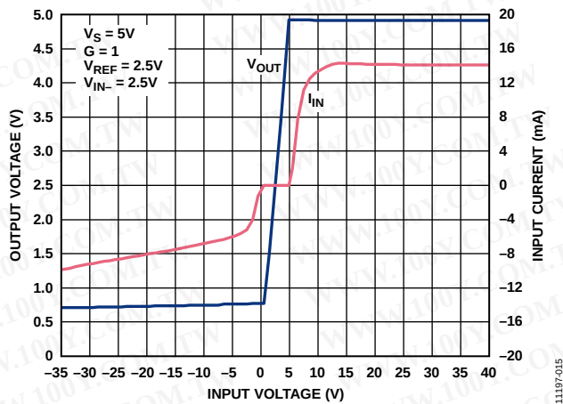
Figure 16. Input Overvoltage Performance; G = 1 , V_S = 5\text{ V}
