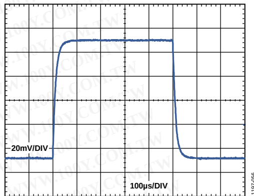
Figure 55. Small Signal Pulse Response ( G = 1000 ), R_L = 2\text{ k}\Omega , C_L = 100\text{ pF}
