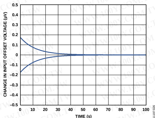
Figure 27. Change in Input Offset Voltage ( V_{OS} ) vs. Warm-Up Time
