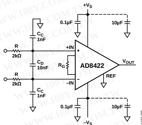
Figure 64. RFI Suppression
