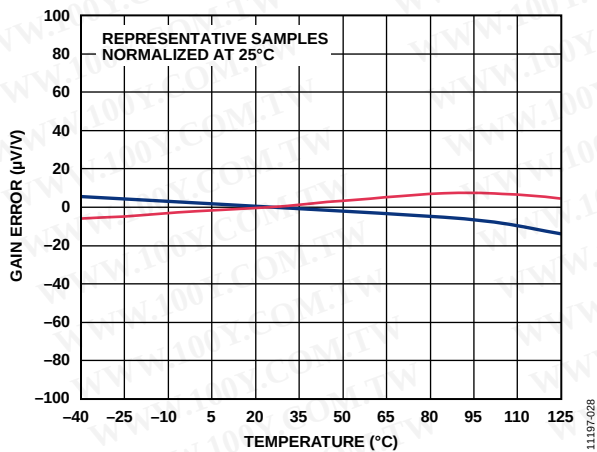
Figure 29. Gain vs. Temperature (G = 1)
