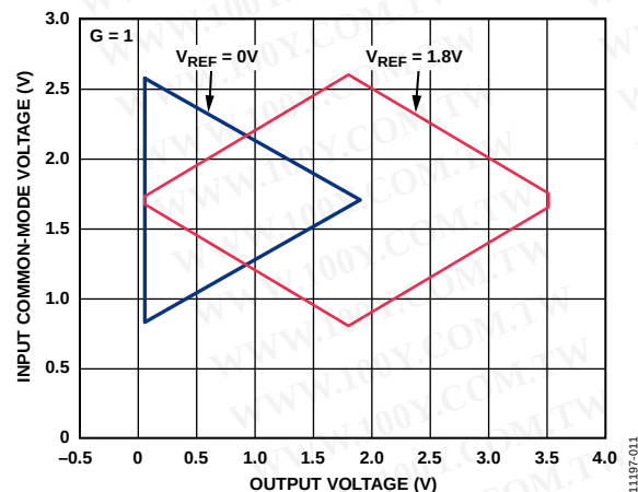
Figure 12. Input Common-Mode Voltage vs. Output Voltage ( G = 1 ), Single-Supply, V_S = 3.6\text{ V}
