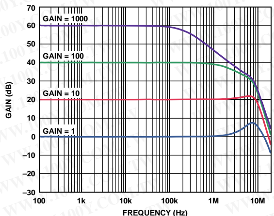
Figure 21. Gain vs. Frequency
