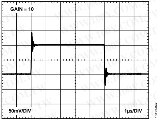
Figure 52. Small Signal Pulse Response ( G = 10 ), R_L = 600\ \Omega , C_L = 100\ \text{pF}
