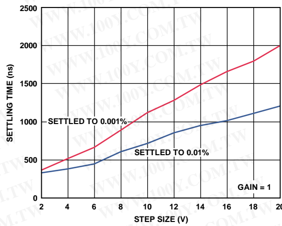
Figure 50. Settling Time vs. Step Size ( G = 1 ), R_L = 2 k \Omega , C_L = 100 pF
