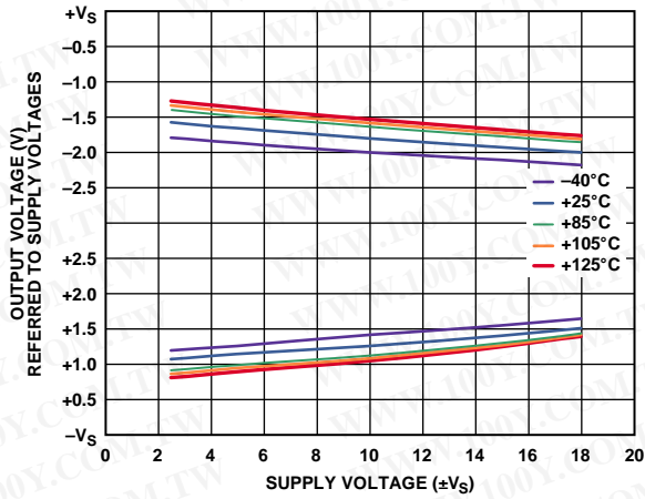
Figure 34. Output Voltage Swing vs. Supply Voltage, R_L = 600\ \Omega
