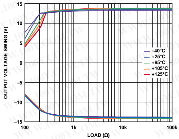
Figure 35. Output Voltage Swing vs. Load Resistance
