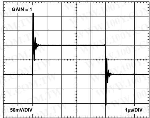
Figure 51. Small Signal Pulse Response ( G = 1 ), R_L = 600 \Omega , C_L = 100 pF
