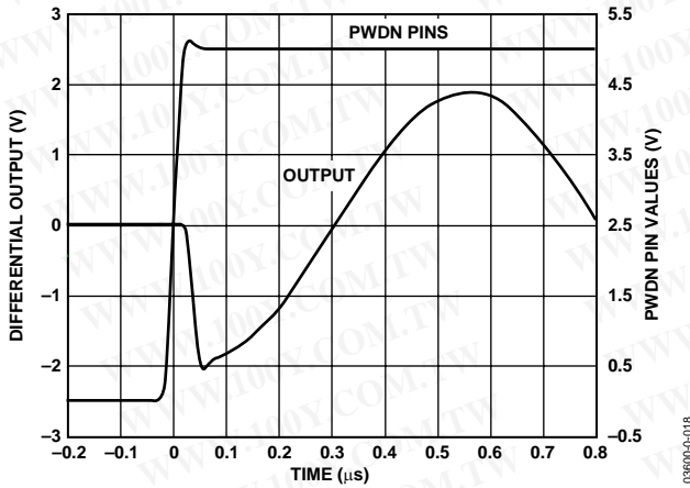
Figure 17. Power-Up Time; PWDN = (0,0) to PWDN = (1,1)
