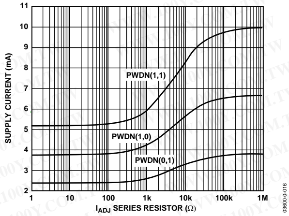
Figure 16. Quiescent Current vs. I_{ADJ} Resistor; V_S = \pm 12 V
