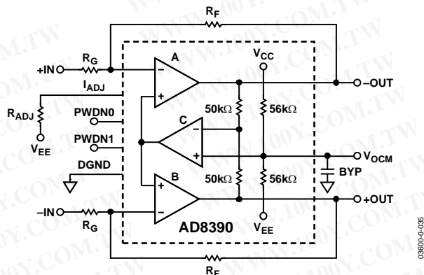
Figure 22. Functional Block Diagram
