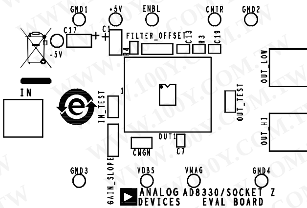
Figure 72. Component-Side Silkscreen
