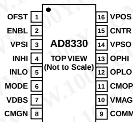
Figure 3. 16-Lead QSOP Pin Configuration
