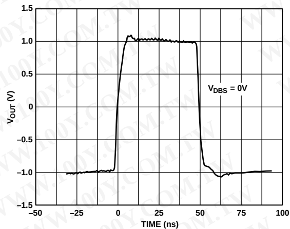
Figure 33. Full-Scale Transient Response, V_{DBS} = 0\text{ V}
