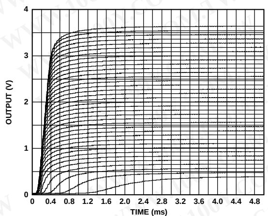
Figure 68. Time Domain Response of RMS Voltmeter (Simulation)
