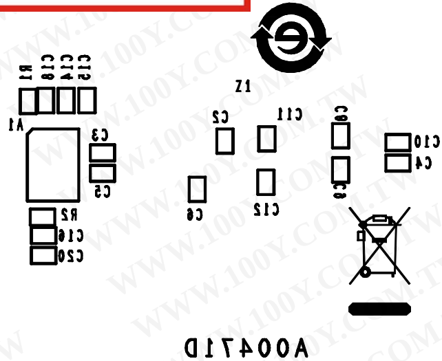
Figure 75. Wiring-Side Silkscreen
