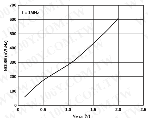
Figure 18. Output Referred Noise vs. V_{MAG} , V_{DDB} = 0.75\text{ V}
