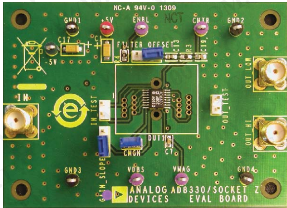
Figure 69. Photograph of the AD8330 Evaluation Board
