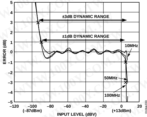
Figure 30. Log Conformance Errors vs. Input Level at 10 MHz, 50 MHz, and 100 MHz
