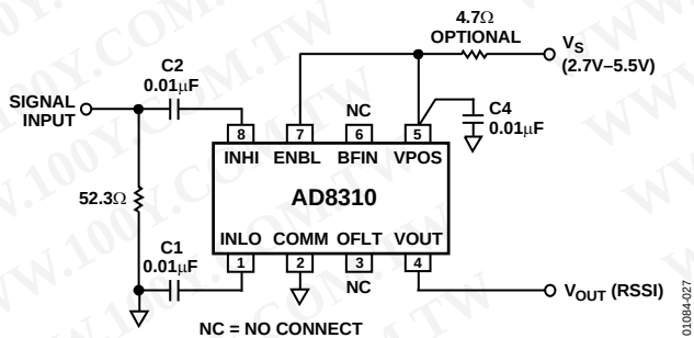
Figure 27. Basic Connections
