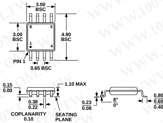
Figure 43. 8-Lead Mini Small Outline Package [MSOP] (RM-8) Dimensions shown in millimeters
