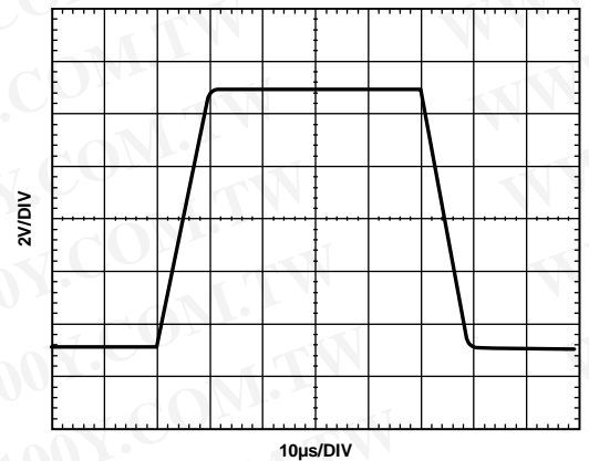
Figure 30. Large-Signal Step Response
