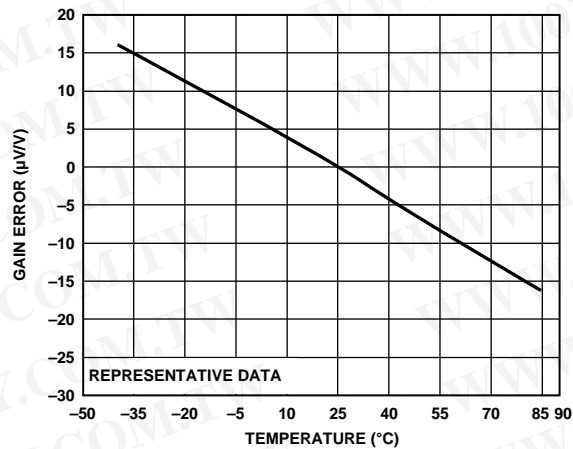
Figure 11. Gain Error vs. Temperature, Normalized at 25°C
