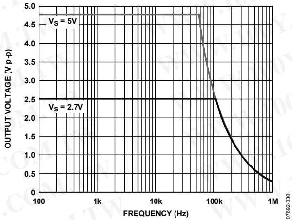
Figure 32. Maximum Output Voltage vs. Frequency, V_S = 5V, 2.7V
