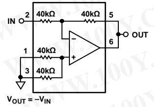
Figure 44. Inverting Amplifier, Gain = -1
