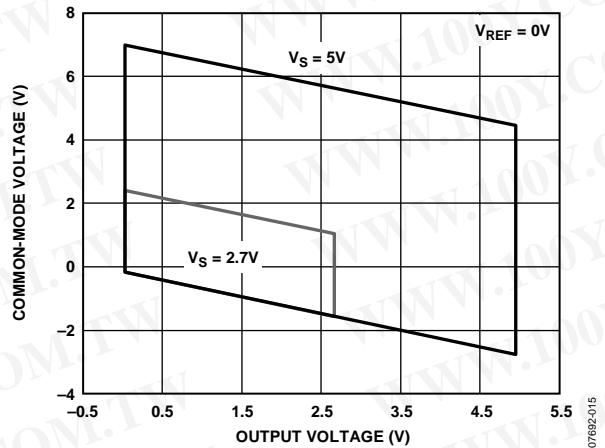
Figure 17. Input Common-Mode Voltage vs. Output Voltage, 5 V and 2.7 V Supplies, V_{REF} = 0\text{ V}
