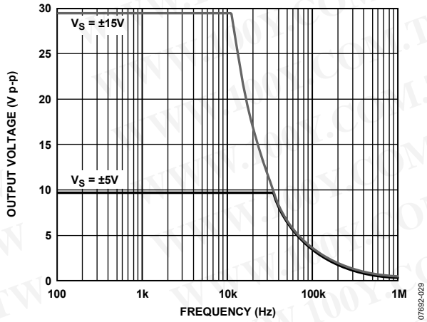
Figure 31. Maximum Output Voltage vs. Frequency, V_S = \pm 15V, \pm 5V
