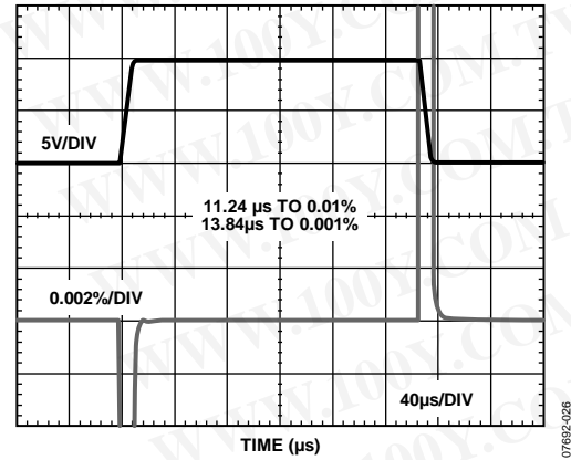
Figure 28. Large-Signal Pulse Response and Settling Time, 10 V Step, V_S = \pm 15 V
