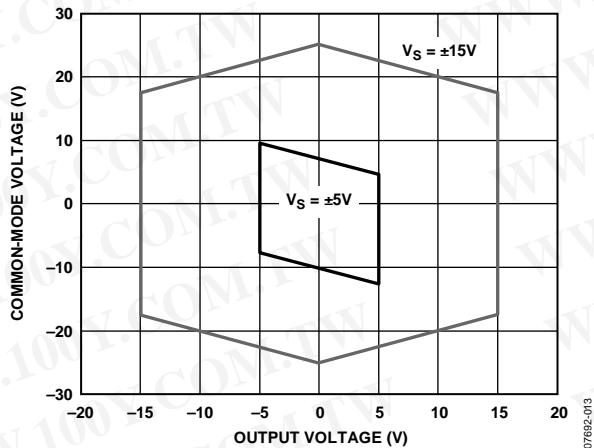
Figure 15. Input Common-Mode Voltage vs. Output Voltage, \pm 15\text{ V} and \pm 5\text{ V} Supplies
