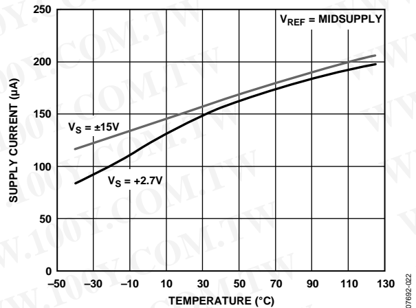
Figure 24. Supply Current Per Channel vs. Temperature
