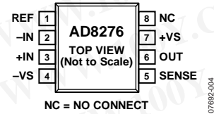
Figure 5. AD8276 8-Lead SOIC Pin Configuration
