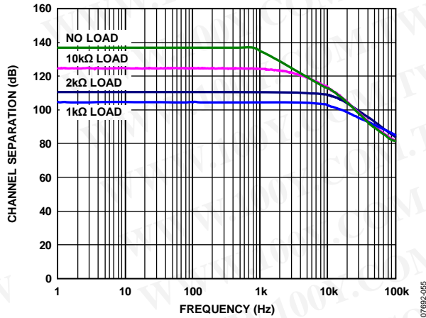
Figure 37. Channel Separation
