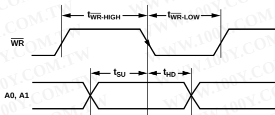
Figure 54. Timing Diagram for Latched Gain Mode
