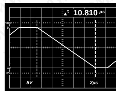
Figure 8. Slew Rate, R_L = 10k
