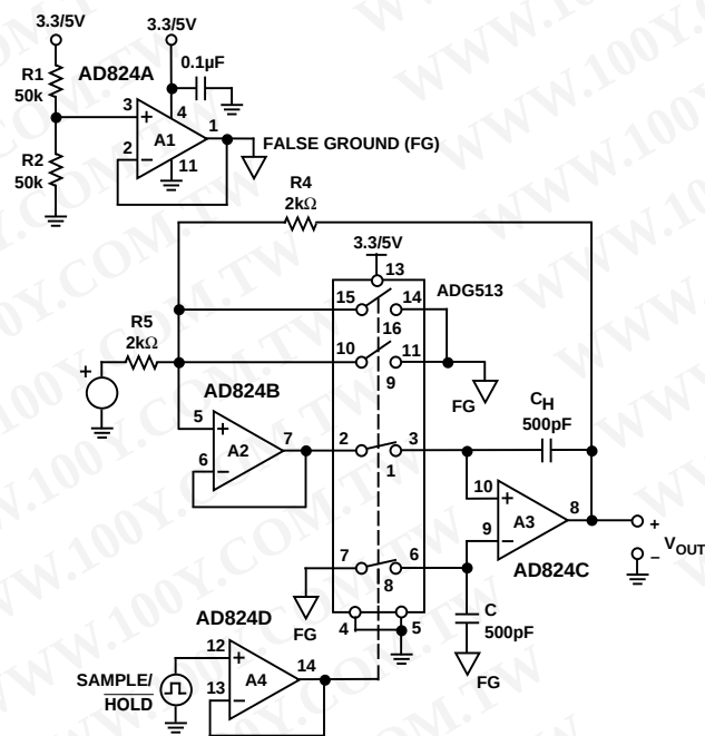
Figure 35. 3.3 V/5 V Precision Sample and Hold
