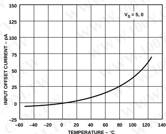
Figure 15. Input Offset Current vs. Temperature
