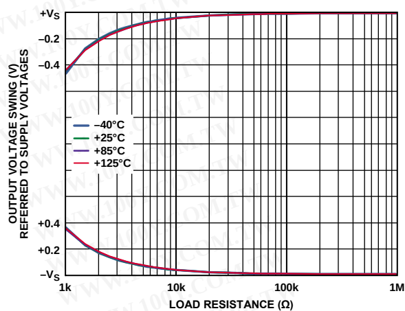
Figure 61. Output Voltage Swing vs. Load Resistance, V_S = \pm 2.5\text{ V}
