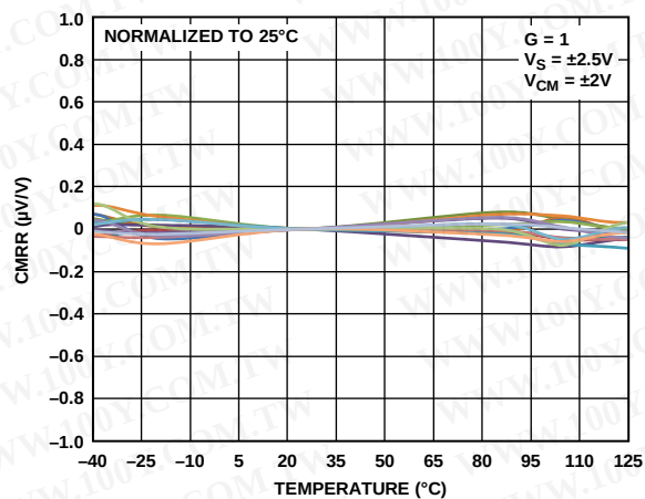
Figure 57. CMRR vs. Temperature
