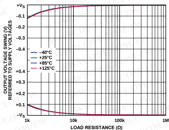
Figure 62. Output Voltage Swing vs. Load Resistance, V_S = \pm 0.9\text{ V}
