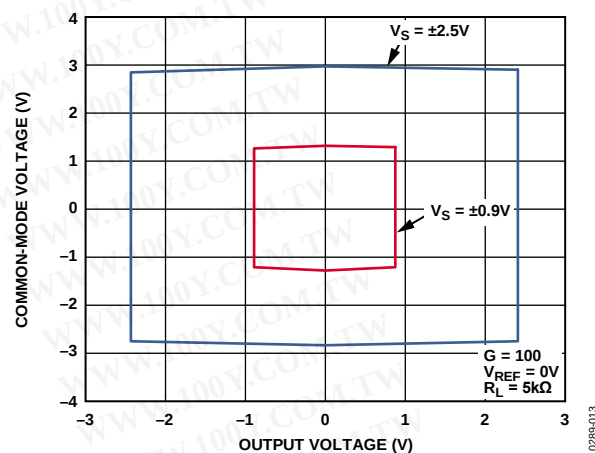
Figure 13. Input Common-Mode Voltage vs. Output Voltage, G = 100 , V_{REF} = 0V , V_S = \pm 2.5V and V_S = \pm 0.9V , R_L = 5k\Omega to Ground
