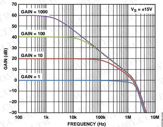
Figure 25. Gain vs. Frequency, V_S = \pm 15 V
