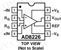
Figure 60. Pinout Diagram
