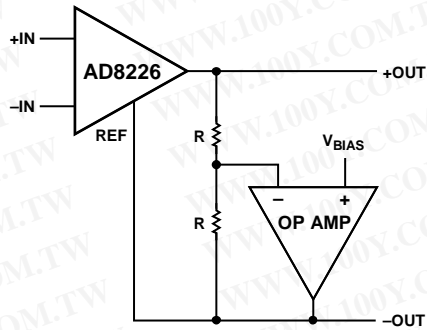
Figure 64. Differential Output Using an Op Amp
