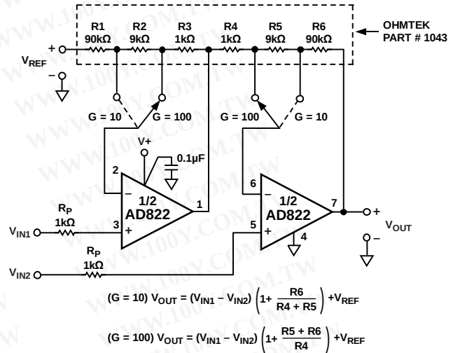
Figure 49. A Single-Supply Programmable Gain Instrumentation Amplifier
