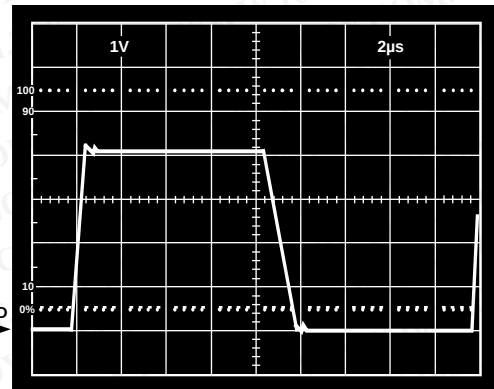
Figure 34. V_S = 5 V , 0 V; Unity-Gain Follower Response to 0 V to 4 V Step
