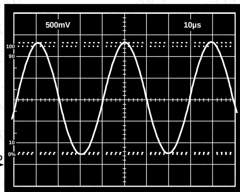
Figure 41. V_S = 3\text{ V} , 0\text{ V} ; Gain-of-2 Inverter, V_{IN} = 1.25\text{ V} , 25\text{ kHz} , Sine Wave Centered at -0.75\text{ V} , R_L = 600\text{ }\Omega
