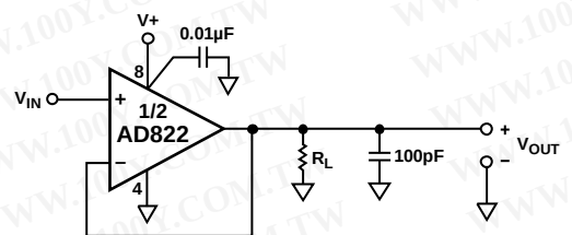
Figure 35. Unity-Gain Follower
