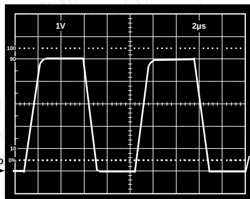
Figure 40. V_S = 5\text{ V} , 0\text{ V} ; Gain-of-2 Inverter Response to 2.5\text{ V} Step, Centered -1.25\text{ V} Below Ground, R_L = 10\text{ k}\Omega
