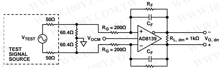
Figure 57. Basic Test Circuit
