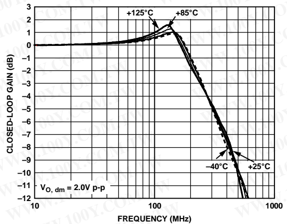
Figure 12. Large Signal Frequency Response at Various Temperatures
