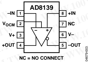
Figure 5. 8-Lead SOIC Pin Configuration
