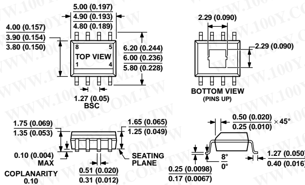
COMPLIANT TO JEDEC STANDARDS MS-012-AA CONTROLLING DIMENSIONS ARE IN MILLIMETER; INCH DIMENSIONS (IN PARENTHESES) ARE ROUNDED-OFF MILLIMETER EQUIVALENTS FOR REFERENCE ONLY AND ARE NOT APPROPRIATE FOR USE IN DESIGN. Figure 65. 8-Lead Standard Small Outline Package with Exposed Pad [SOIC_N_EP] Narrow Body (RD-8-1)—Dimensions shown in millimeters and (inches)
