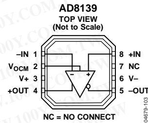
Figure 6. 8-Lead LFCSF Pin Configuration
