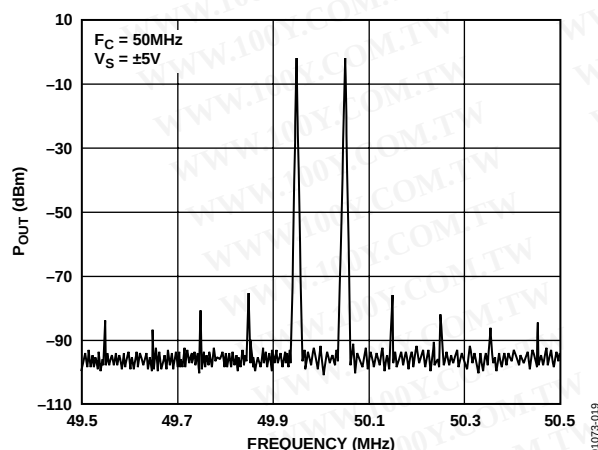
Figure 19. Intermodulation Distortion
