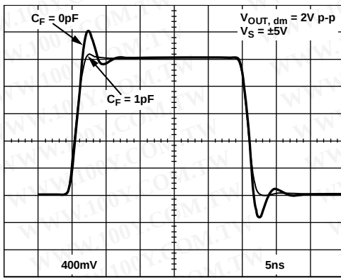
Figure 24. Large Signal Transient Response
