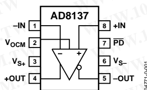
Figure 4. Pin Configuration
