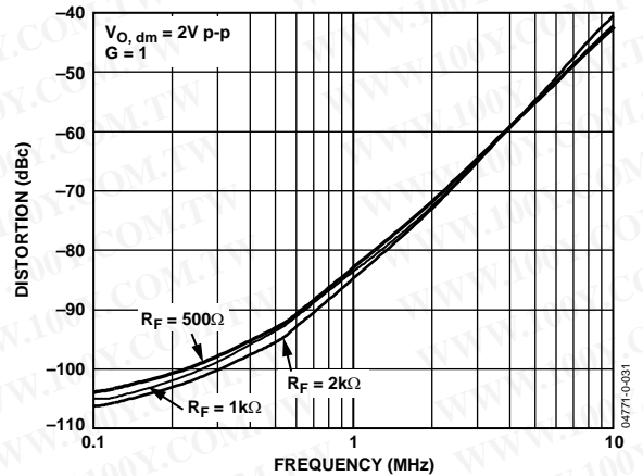
Figure 28. Third Harmonic Distortion at Various R_F
