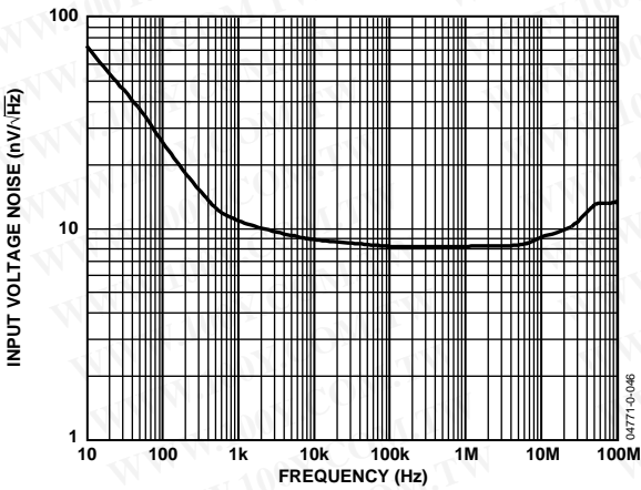
Figure 30. Input Voltage Noise vs. Frequency
