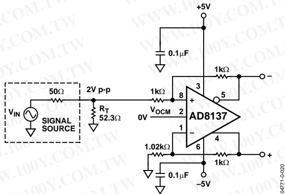
Figure 67. AD8137 with Terminated Input
