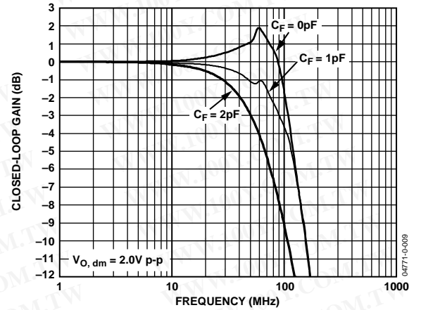
Figure 15. Large Signal Frequency Response for Various C_F
