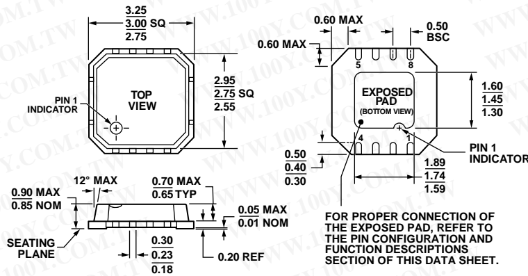
Figure 73. 8-Lead Lead Frame Chip Scale Package [LFCSF_VD] 3 mm x 3 mm Body, Very Thin, Dual Lead (CP-8-2)
