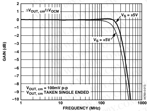
Figure 26. V_{OCM} Frequency Response for Various Power Supply Voltages
