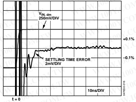
Figure 17. Settling Time (0.1%)
