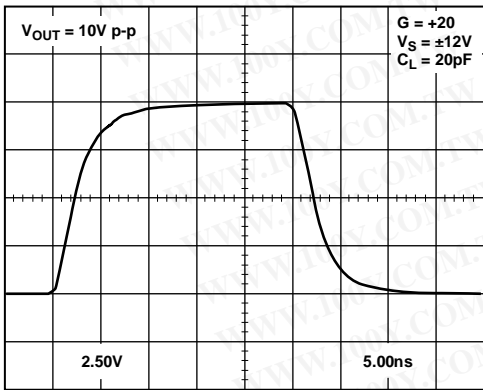
Figure 109. AD8129 Transient Response, V_{OUT} = 10V p-p, G = +20
