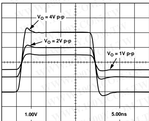
Figure 103. Transient Response vs. Output Amplitude, V_{OUT} = 1\text{ V p-p}, 2\text{ V p-p}, 4\text{ V p-p}
