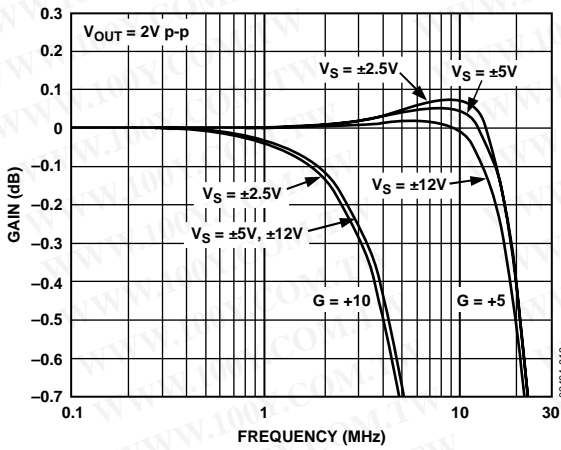
Figure 18. AD8130 Fine Scale Response vs. Supply, G = +5 , G = +10 , V_{OUT} = 2\ V\ p-p
