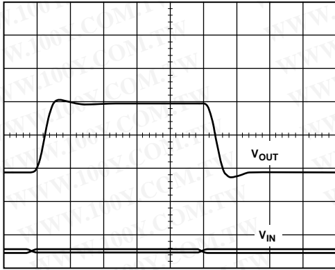
Figure 108. AD8129 Transient Response with -3.5 V Common-Mode Input
