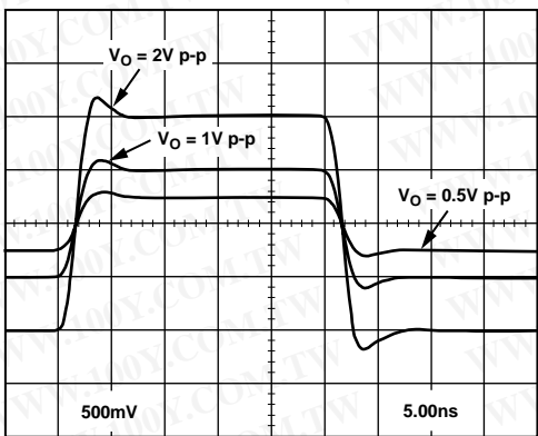
Figure 102. Transient Response vs. Output Amplitude, V_{OUT} = 0.5\text{ V p-p}, 1\text{ V p-p}, 2\text{ V p-p}
