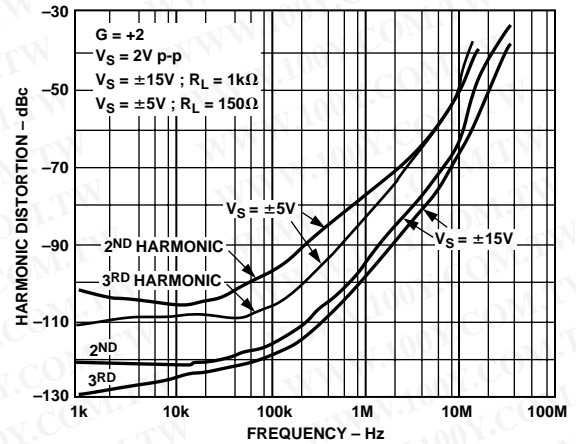
Figure 20. Harmonic Distortion vs. Frequency
