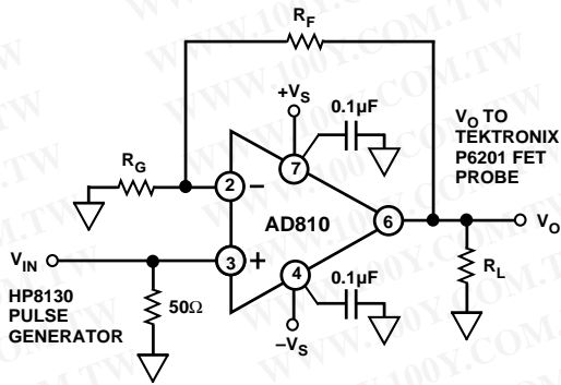
Figure 19. Noninverting Amplifier Connection
