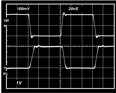
Figure 37. Small Signal Pulse Response, Gain = -10, R_F = 442 \Omega , R_L = 150 \Omega , V_S = \pm 15 V
