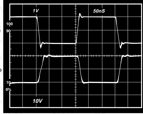
Figure 38. Large Signal Pulse Response, Gain = -10, R_F = 442 \Omega , R_L = 400 \Omega , V_S = \pm 15 V
