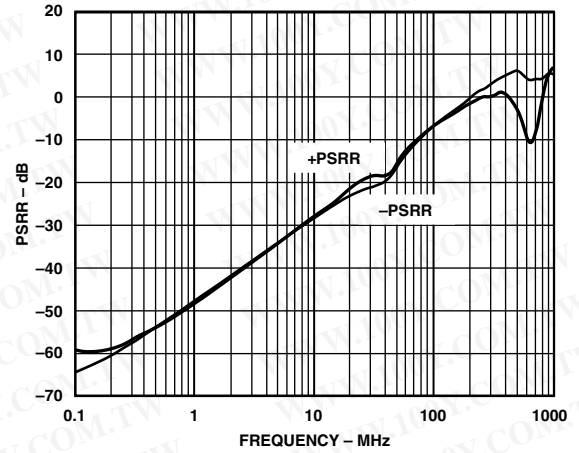
TPC 15. AD8075 PSRR vs. Frequency
