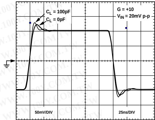
Figure 19. Small Signal Transient Response \pm 5\text{V} Supply
