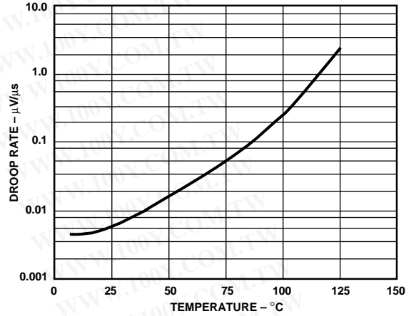
Droop Rate vs. Temperature, V_{IN} = 0\text{ V}
