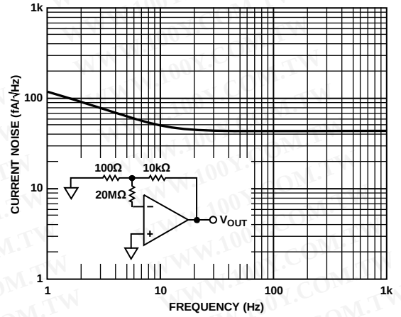
Figure 17. Input Noise Current Spectral Density
