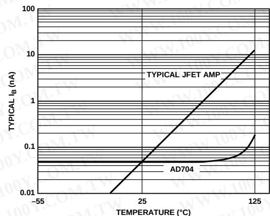
Figure 4. Input Bias Current Over Temperature
