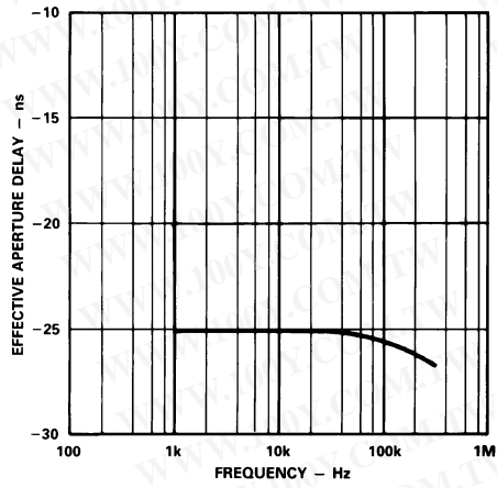
Effective Aperture Delay vs. Frequency
