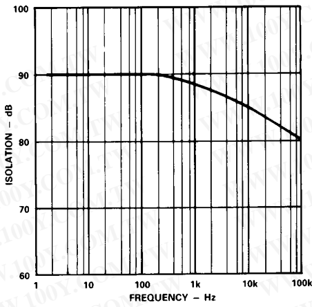
Interchannel Isolation vs. Frequency
