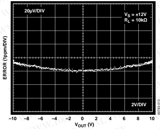
Figure 12. Gain Nonlinearity; V S = ±12 V, R L = 10 kΩ
