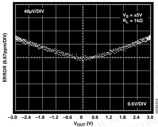
Figure 13. Gain Nonlinearity; V S = ±5 V, R L = 1 kΩ
