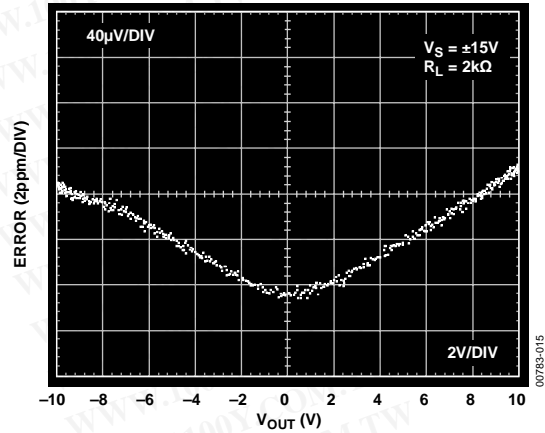
Figure 14. Gain Nonlinearity; V S = ±15 V, R L = 2 kΩ
