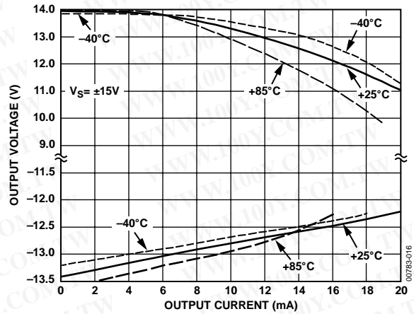
Figure 15. Output Voltage Operating Range vs. Output Current; V S = ±15 V
