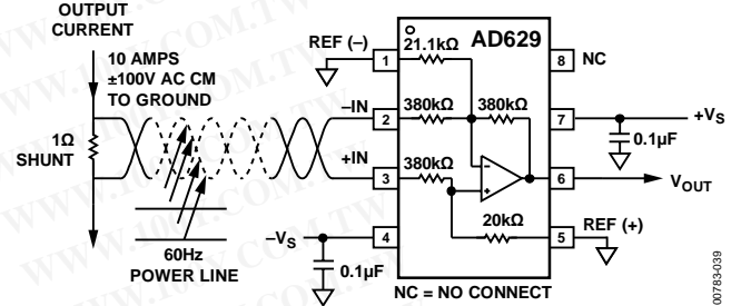
Figure 39. Error Budget Analysis Example 2: V_{IN} = 10 V Full-Scale, V_{CM} = \pm 100 V at 500 Hz, R_{SHUNT} = 1 \Omega
