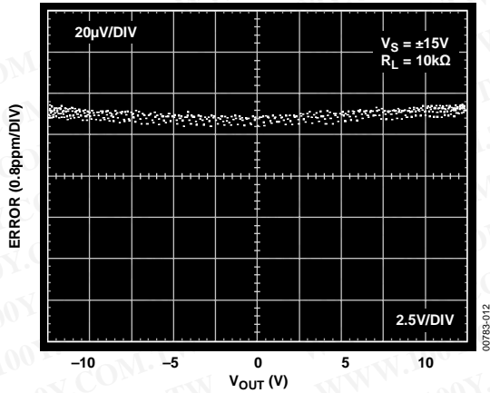
Figure 11. Gain Nonlinearity; V S = ±15 V, R L = 10 kΩ
