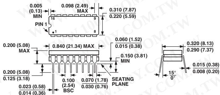
16-Lead Cerdip Package (Q-16)
