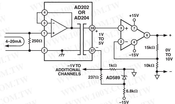
Figure 18. Process Current Input Isolator with Offset
