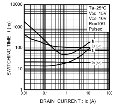
Fig.9 Switching Characteristics
