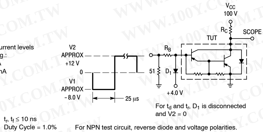
Figure 2. Switching Times Test Circuit
