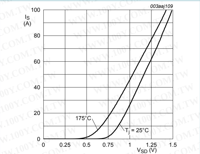
Fig. 17. Source-drain (diode forward) current as a function of source-drain (diode forward) voltage; typical values
