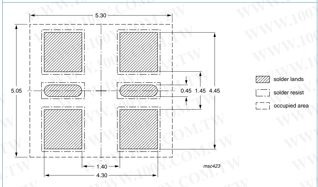
Fig 16. Reflow soldering footprint SOT457 (SC-74)
