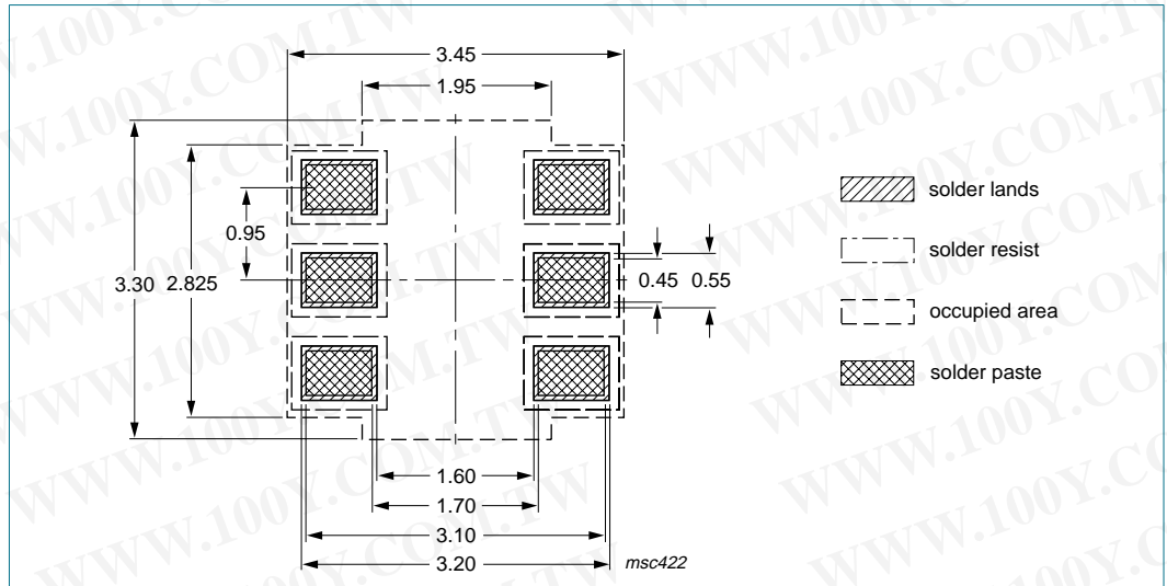
Fig 16. Reflow soldering footprint SOT457 (SC-74)
