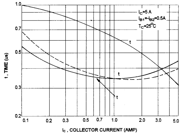
TYPICAL SWITCHING TIME
