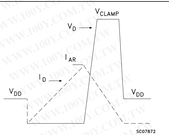
Figure 6. Unclamped inductive waveforms (SC07872)
