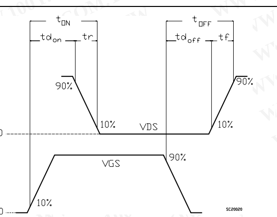
Figure 20. Switching time waveform
