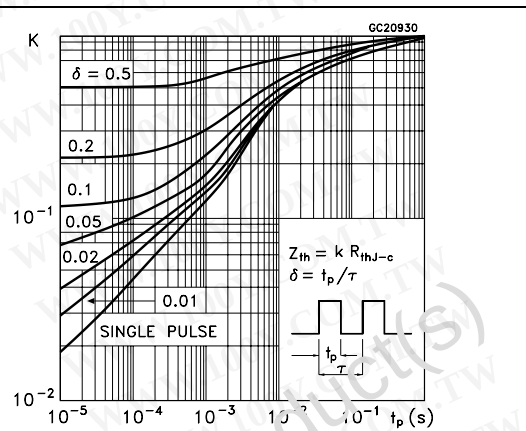
Figure 4. Thermal impedance for TO-220
