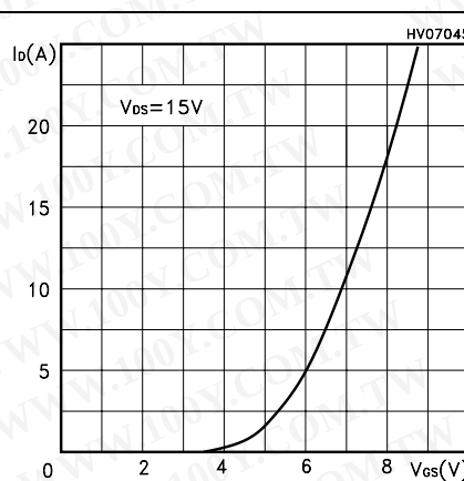
Figure 6. Transfer characteristics
