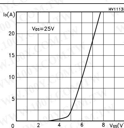
Figure 7. Transfer characteristics
