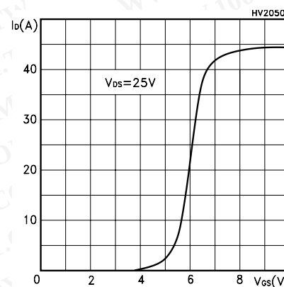
Figure 4. Transfer characteristics
