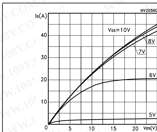
Figure 3. Output characteristics
