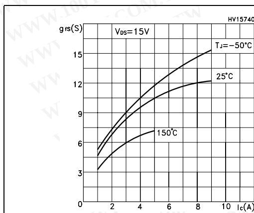
Figure 5. Transconductance
