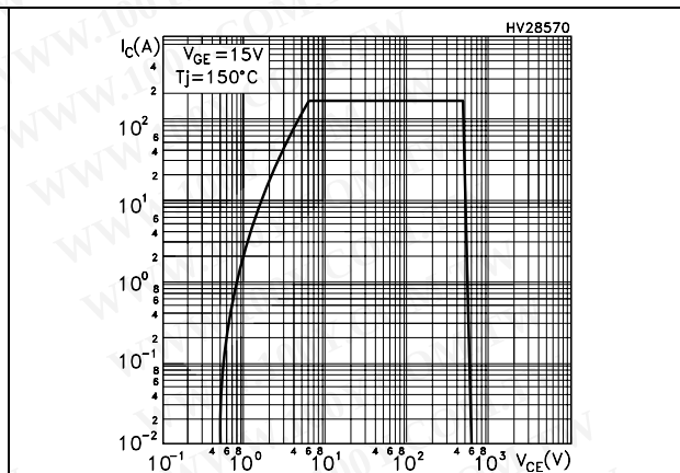
Figure 15. Turn-off SOA
