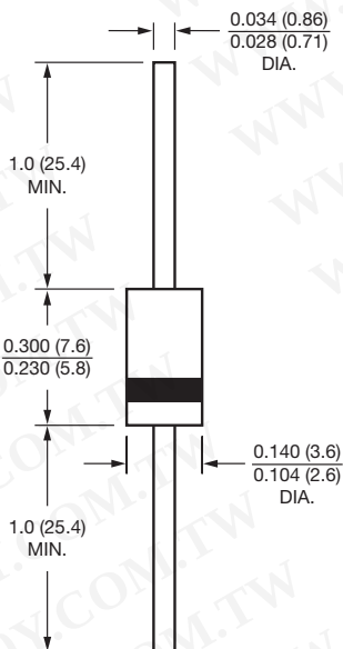
DO-204AC (DO-15)
