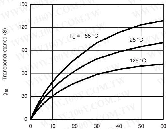
Transconductance
